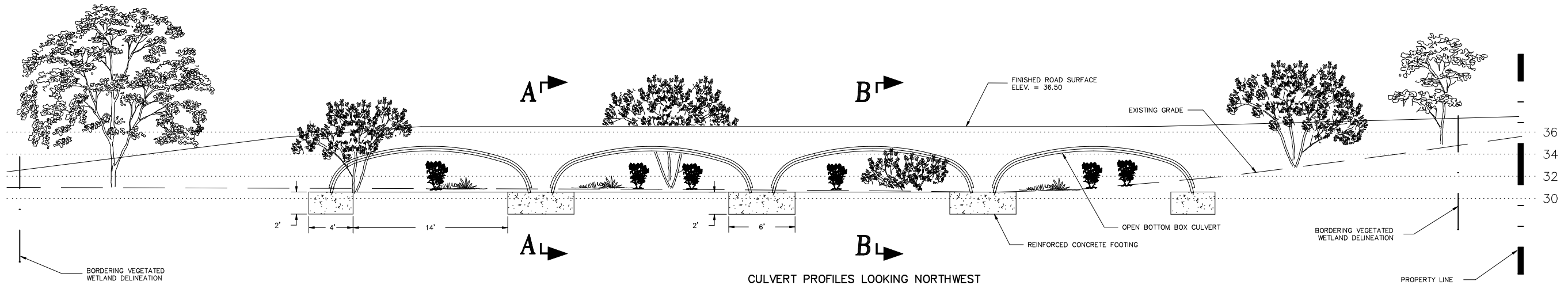
CULVERT PROFILES LOOKING NORTHWEST HORIZONTAL AND VERTICAL SCALE: 1" = 10'
